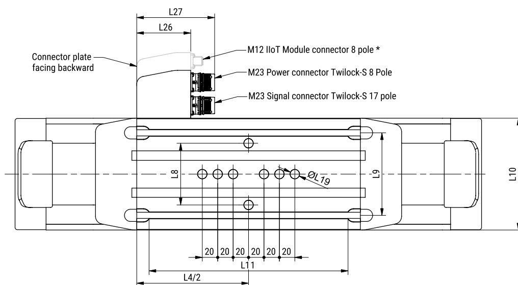
Carriage of the CTL 250
