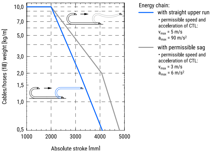
Energy chain overloading and permissible speed/acceleration
