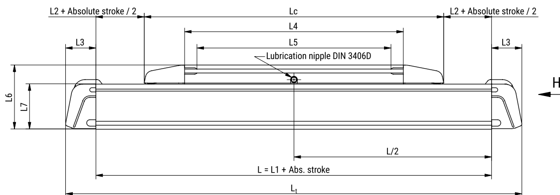
Carriage of the CTL 145 and CTL 200
